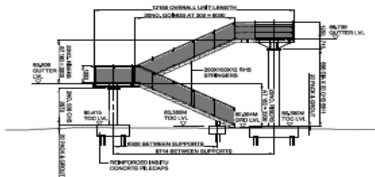
WEST ELEVATION B-B SCALE 1:100
