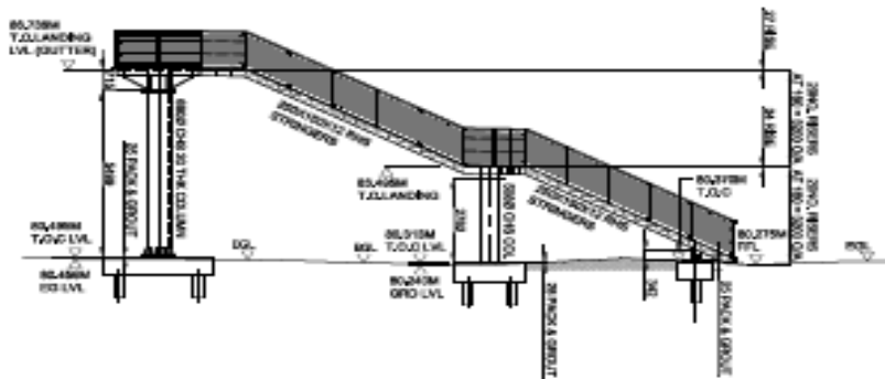
EAST ELEVATION A-A SCALE 1:100
